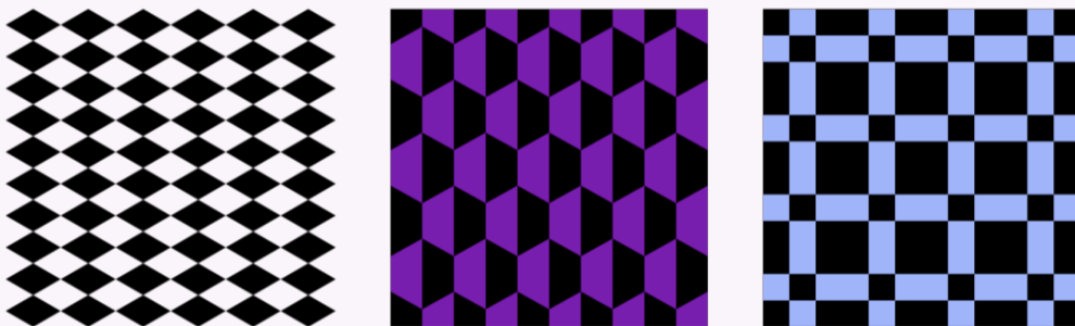
Examples of tessellations using polygons (rhombuses, trapezoids/ hexagons, squares)
